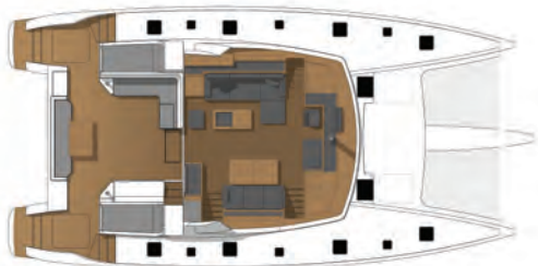
LOUNGE main deck
